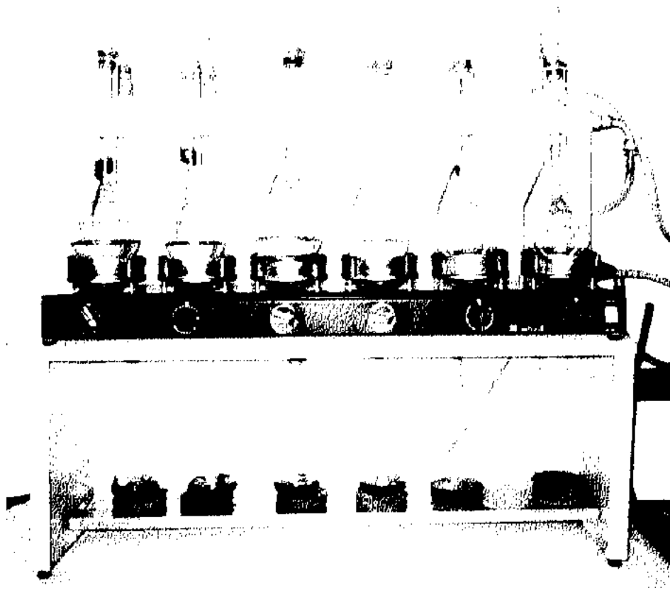
Fig. 1: Macro Kjeldhal distillation apparatus (for protein and NPN and TN analysis)
